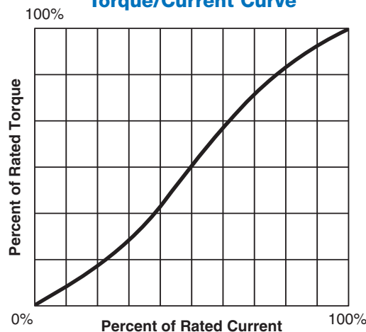
Torque/Current Curve
